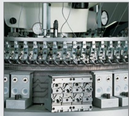
I3P284 – 2+2 cam tracks
