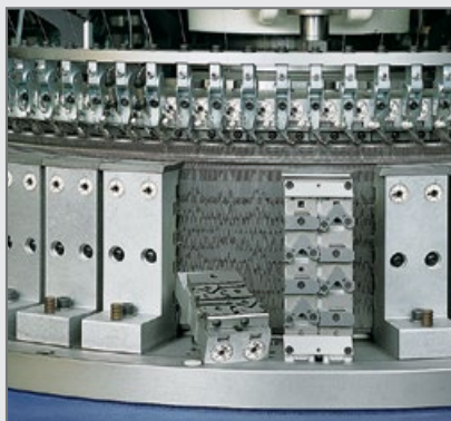
I3P184 – 2+4 cam tracks
