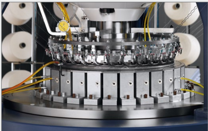
RH216 – knitting head
