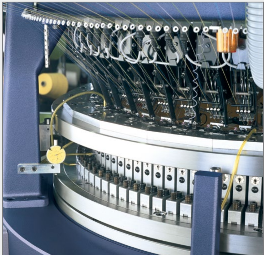
S4F348 – knitting head
