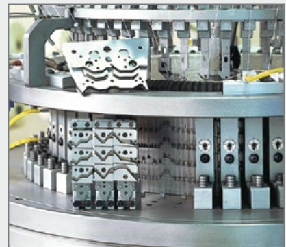
SBF130 – sinker cam and cylinder cam 3-Thread-Fleece
