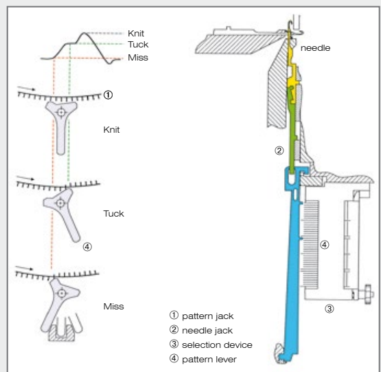
Mini-Jacquard – selection mechanism
